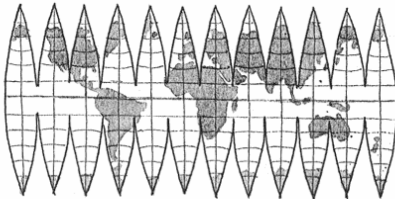
Orange Peel of Globe (Interrupted Sinusoidal Projection)
