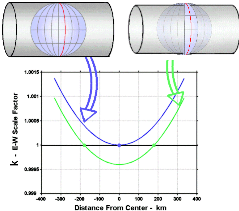
Transverse Mercator Error at Equator — UTM - Depressed In Earth — TM - Tangent To Earth
