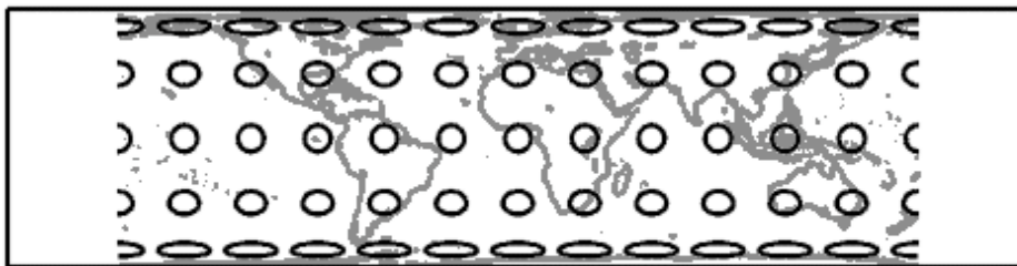
Cylindrical Equal Area
